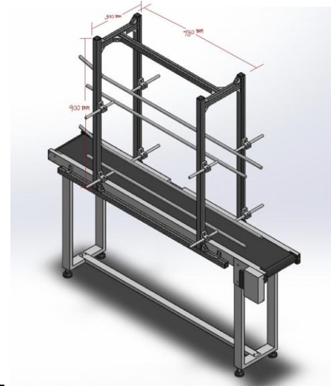
Carton Feeder Type
